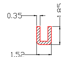
B-B SEC
